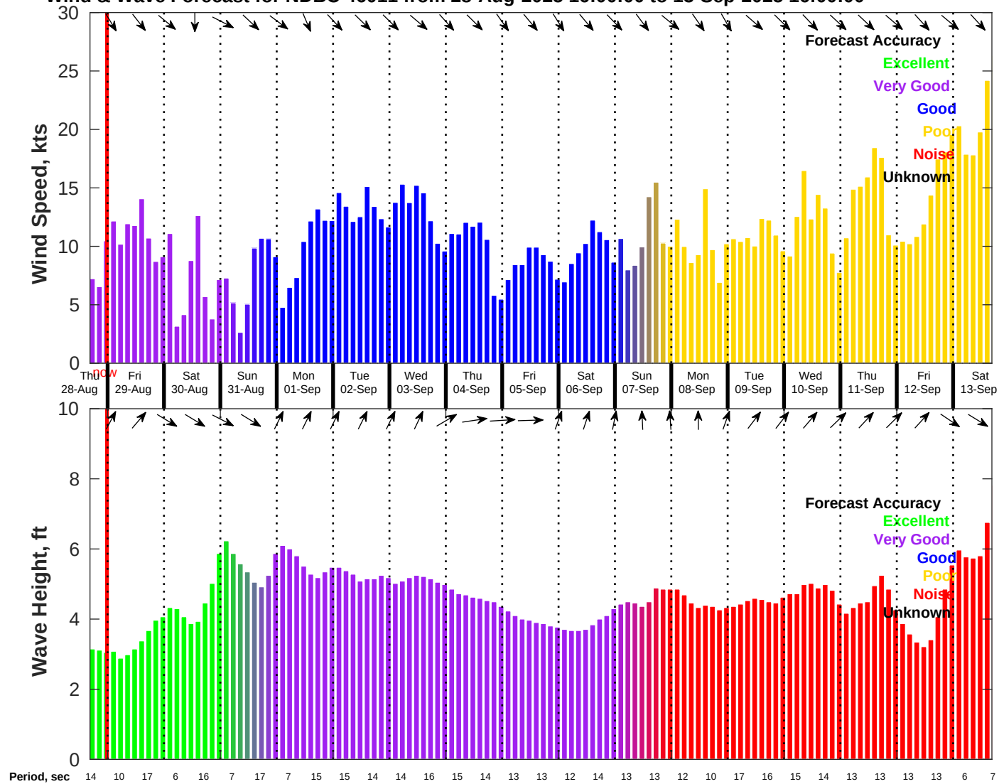
Wind & Wave Forecast for NDBC 46011 from 28-Aug-2025 16:00:00 to 13-Sep-2025 16:00:00
