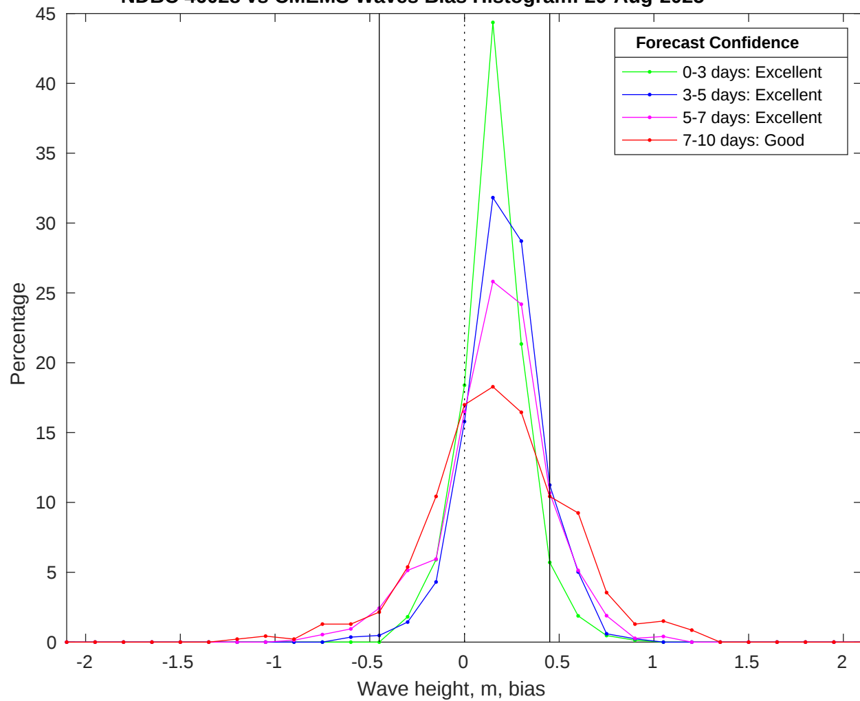
NDBC 46028 vs CMEMS Waves Bias Histogram: 29-Aug-2025
