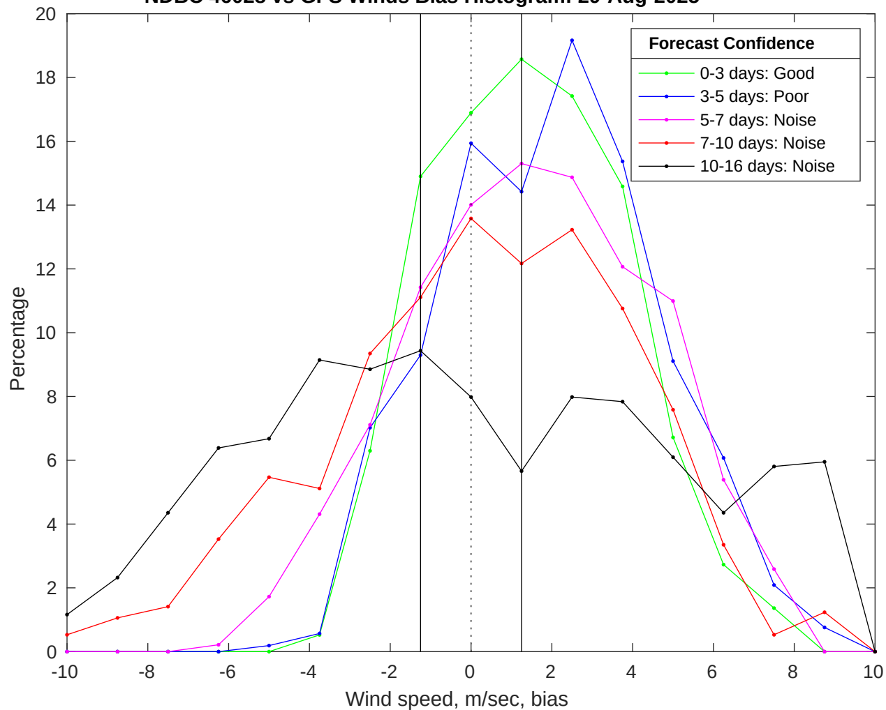
NDBC 46028 vs GFS Winds Bias Histogram: 29-Aug-2025
