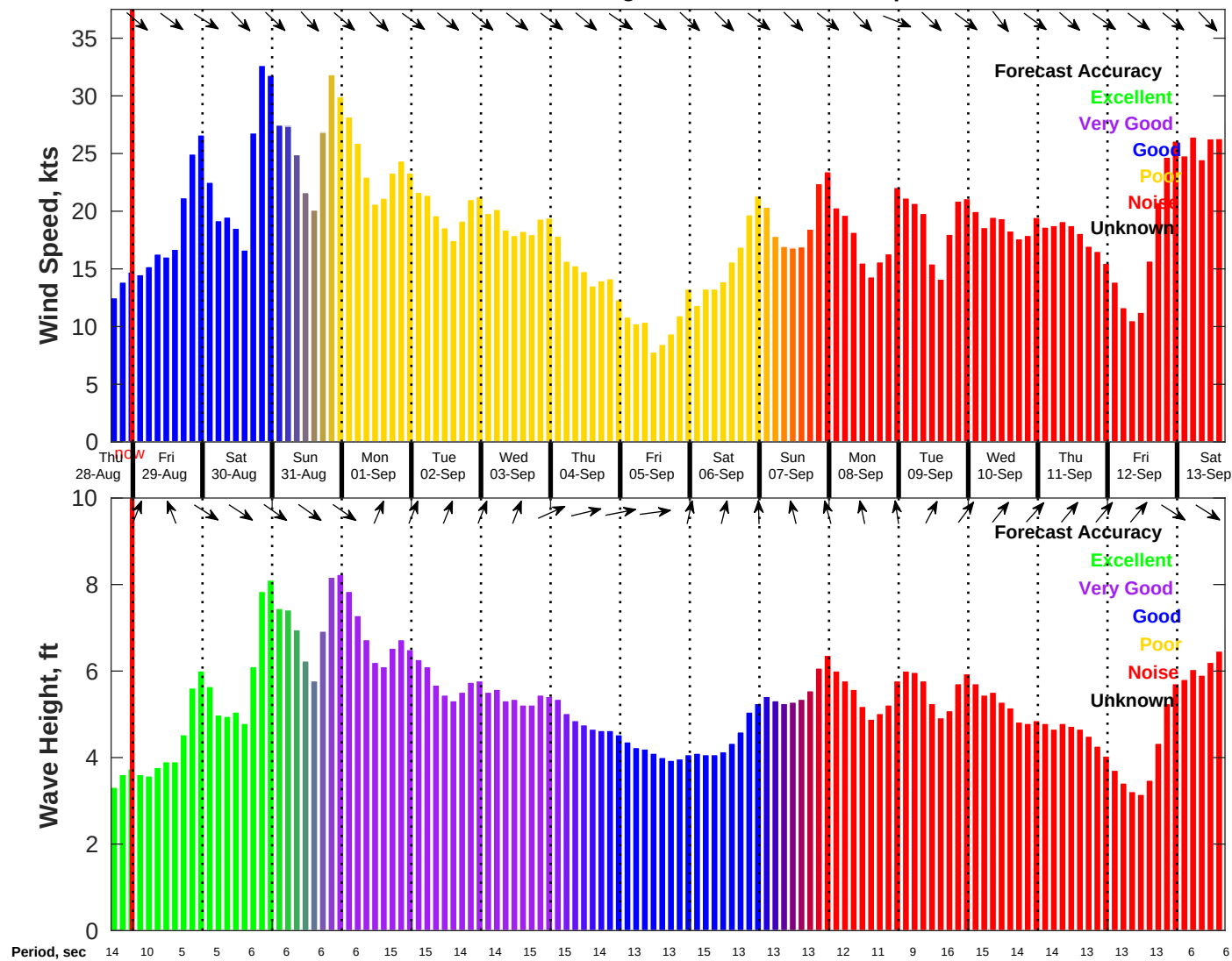
Wind & Wave Forecast for NDBC 46028 from 28-Aug-2025 16:00:00 to 13-Sep-2025 16:00:00
