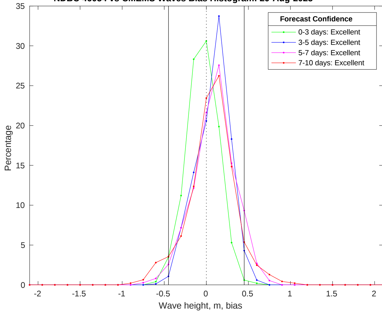
NDBC 46054 vs CMEMS Waves Bias Histogram: 29-Aug-2025
