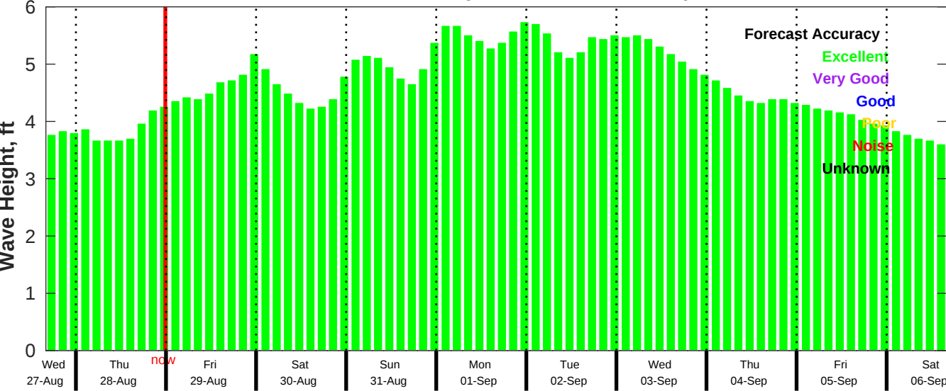
CMEMS Wave Forecast for NDBC 46054 from 27-Aug-2025 16:00:00 to 06-Sep-2025 16:00:00
