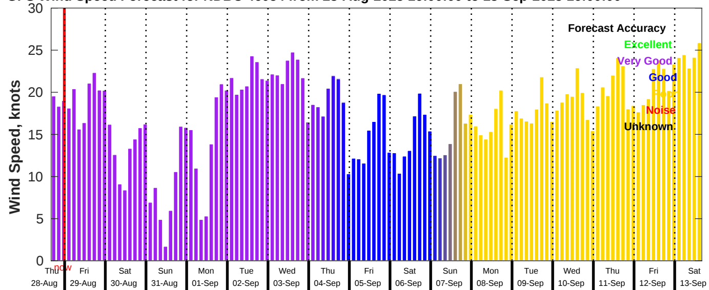
GFS Wind Speed Forecast for NDBC 46054 from 28-Aug-2025 16:00:00 to 13-Sep-2025 16:00:00
