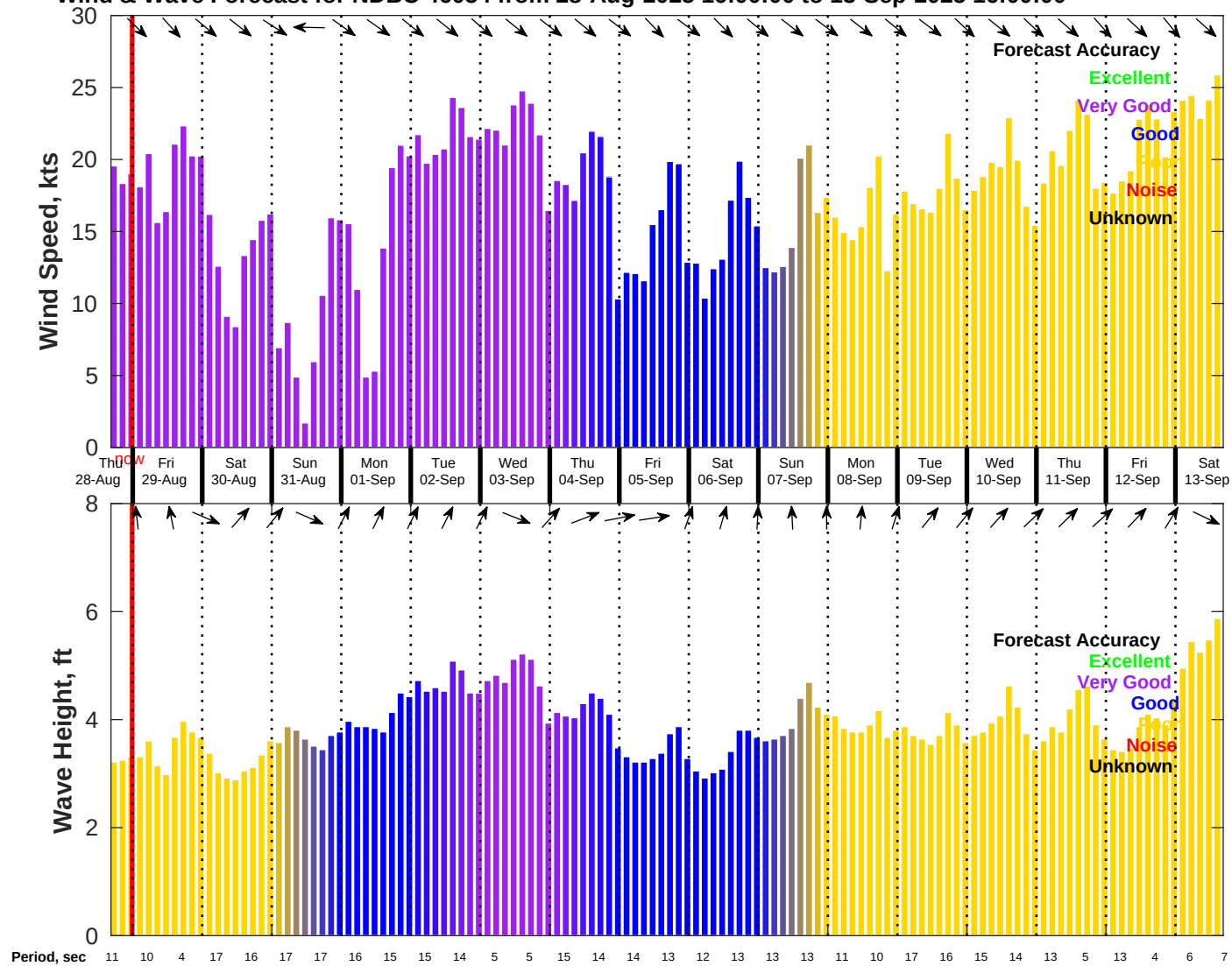
Wind & Wave Forecast for NDBC 46054 from 28-Aug-2025 16:00:00 to 13-Sep-2025 16:00:00
