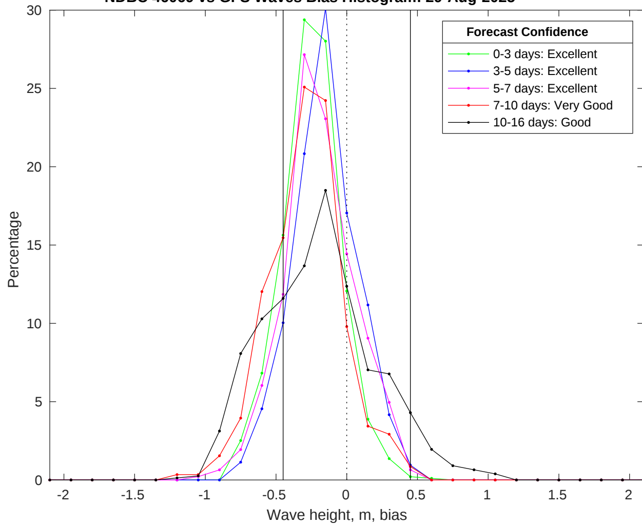
NDBC 46069 vs GFS Waves Bias Histogram: 29-Aug-2025
