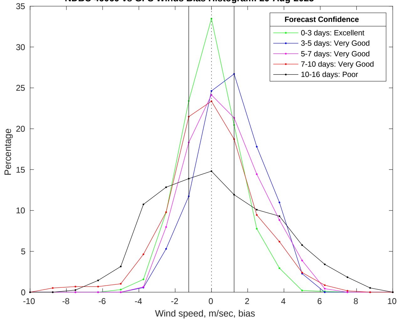
NDBC 46069 vs GFS Winds Bias Histogram: 29-Aug-2025
