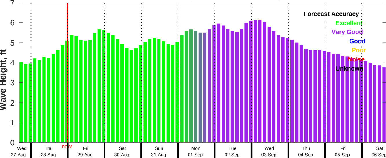
CMEMS Wave Forecast for NDBC 46069 from 27-Aug-2025 16:00:00 to 06-Sep-2025 16:00:00
