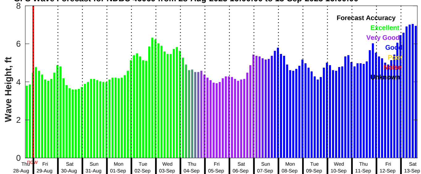
GFS Wave Forecast for NDBC 46069 from 28-Aug-2025 16:00:00 to 13-Sep-2025 16:00:00
