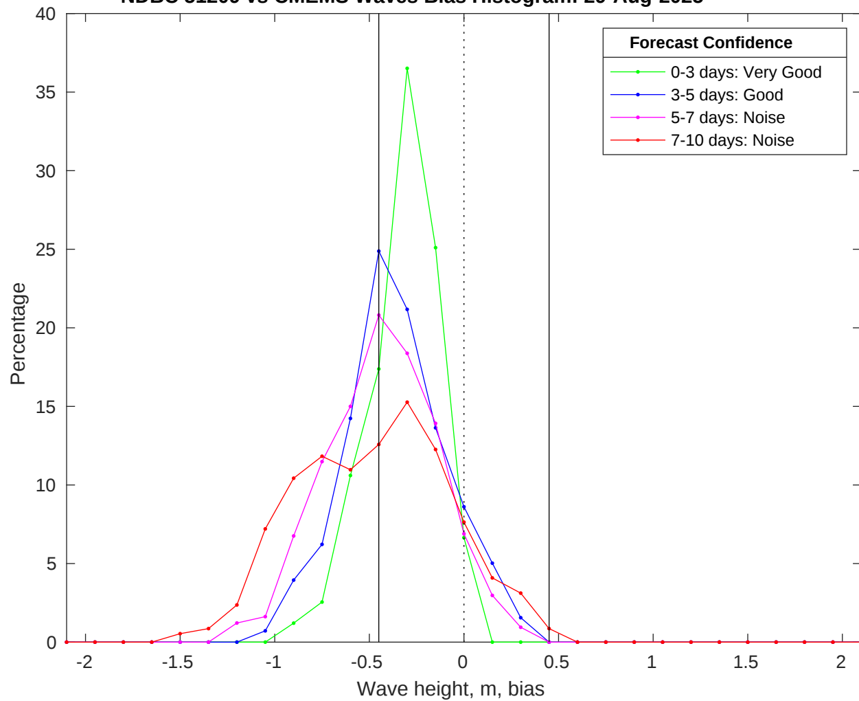
NDBC 51209 vs CMEMS Waves Bias Histogram: 29-Aug-2025
