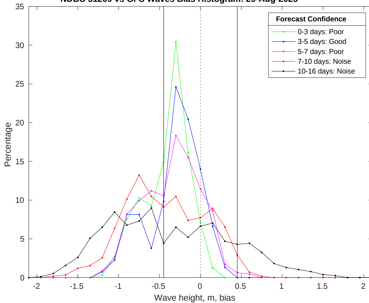
NDBC 51209 vs GFS Waves Bias Histogram: 29-Aug-2025
