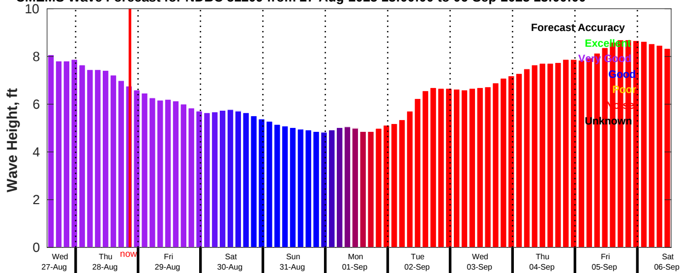
CMEMS Wave Forecast for NDBC 51209 from 27-Aug-2025 13:00:00 to 06-Sep-2025 13:00:00
