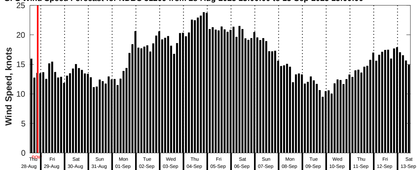
GFS Wind Speed Forecast for NDBC 51209 from 28-Aug-2025 13:00:00 to 13-Sep-2025 13:00:00
