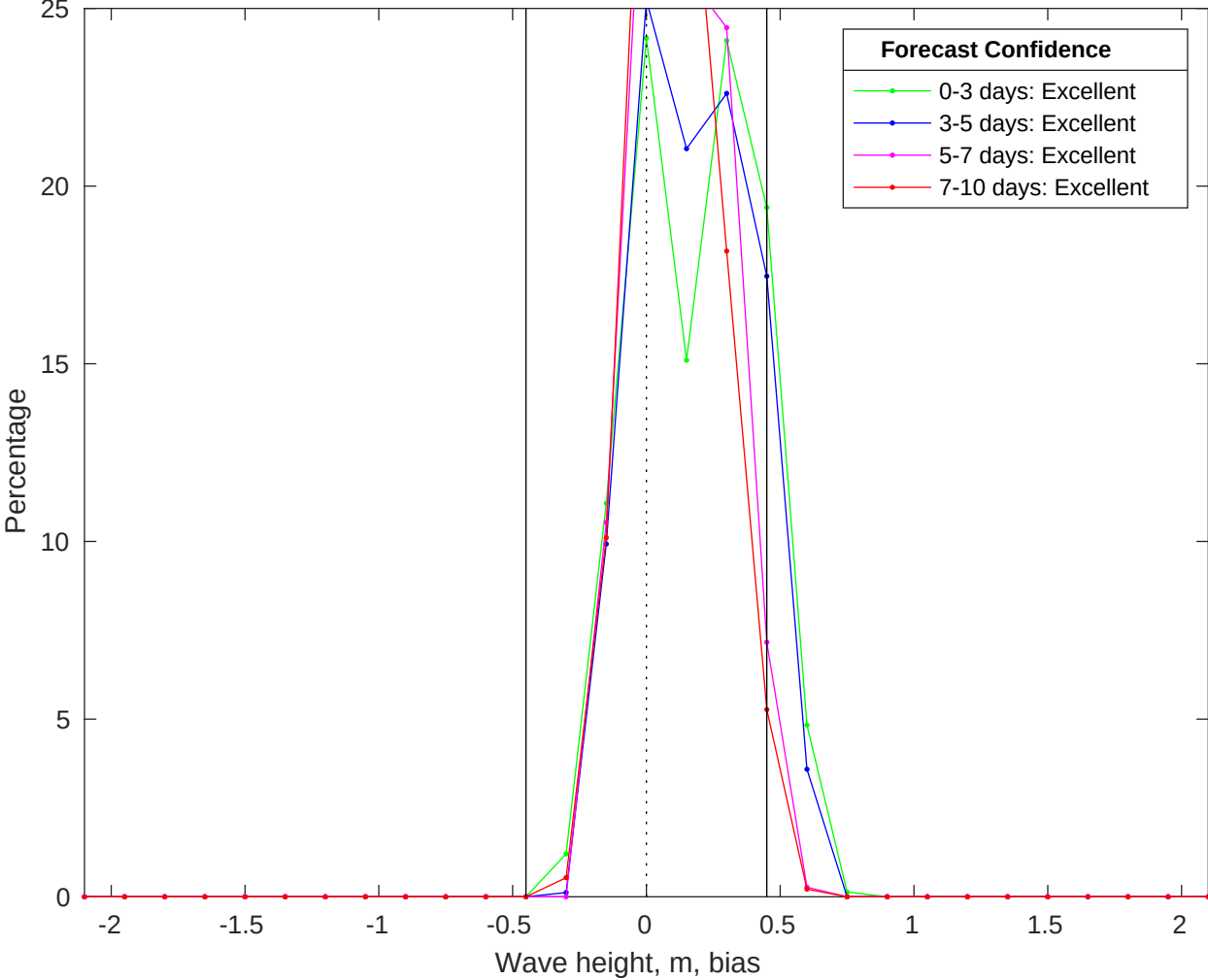
NDBC 51211 vs CMEMS Waves Bias Histogram: 29-Aug-2025
