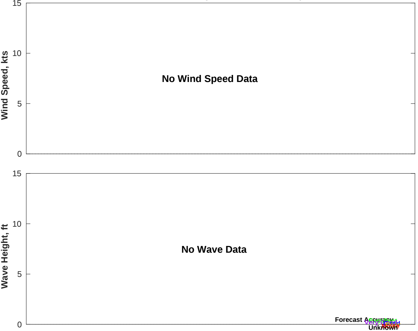
Wind & Wave Forecast for NDBC 51211 from 28-Aug-2025 14:00:00 to 13-Sep-2025 14:00:00
