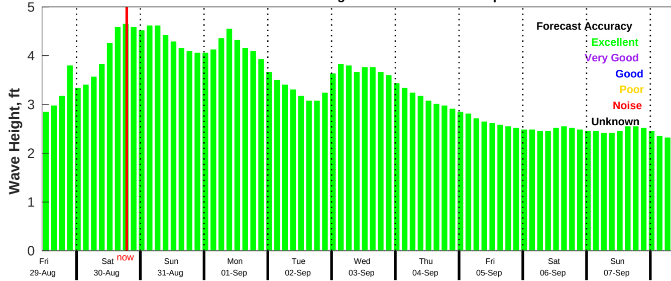
CMEMS Wave Forecast for NDBC 52211 from 28-Aug-2025 11:00:00 to 07-Sep-2025 11:00:00
