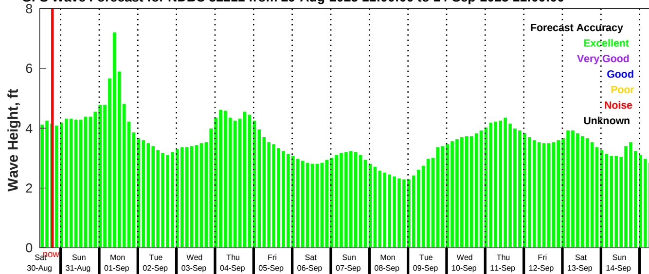
GFS Wave Forecast for NDBC 52211 from 29-Aug-2025 11:00:00 to 14-Sep-2025 11:00:00
