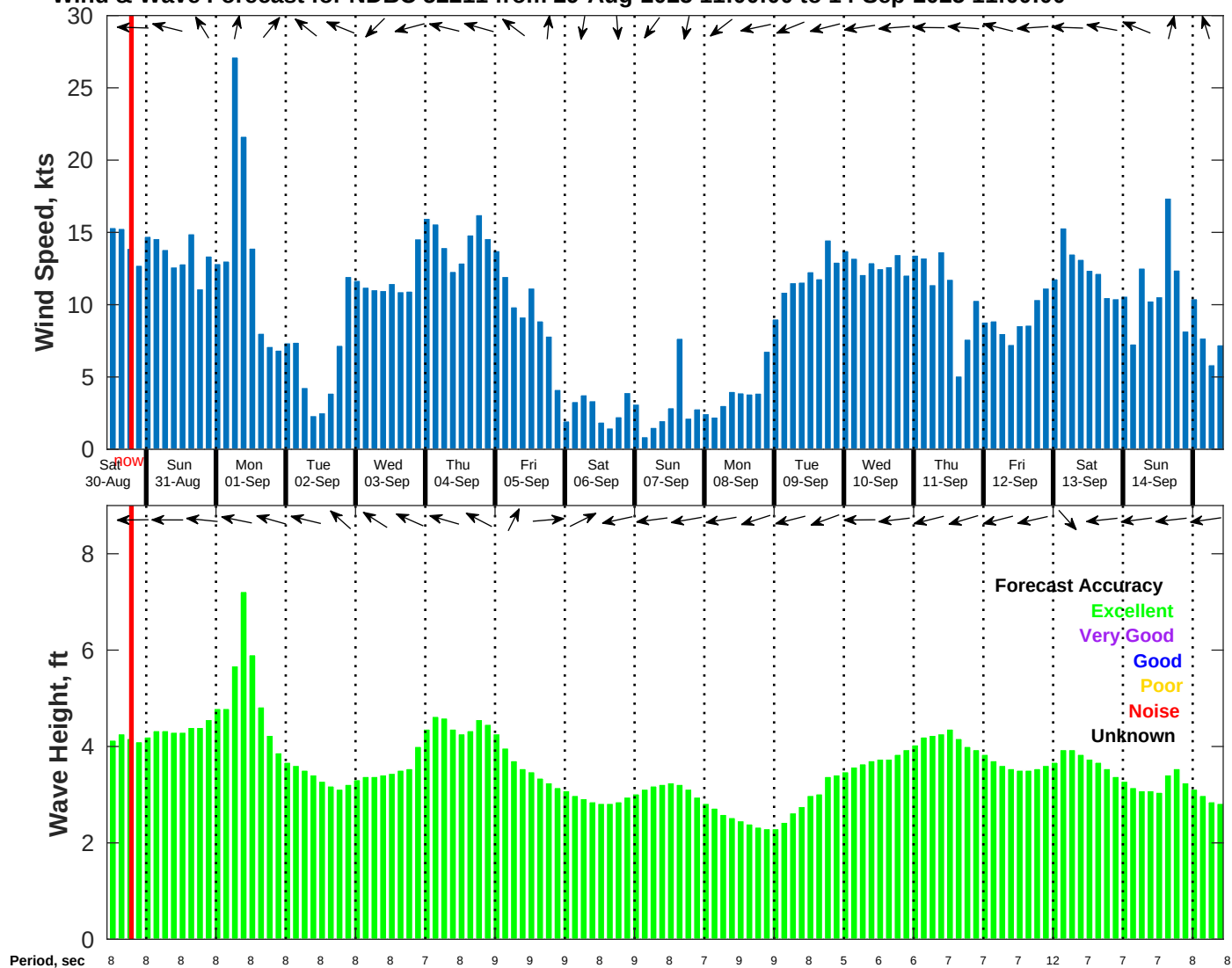
Wind & Wave Forecast for NDBC 52211 from 29-Aug-2025 11:00:00 to 14-Sep-2025 11:00:00
