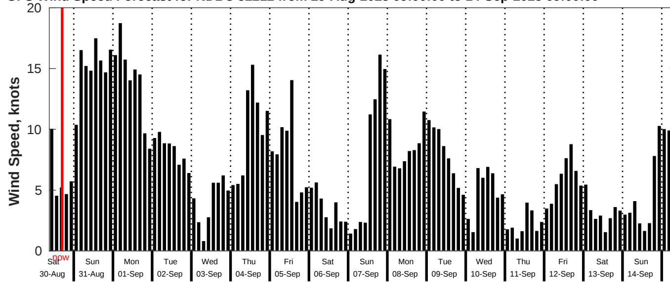
GFS Wind Speed Forecast for NDBC 52212 from 29-Aug-2025 09:00:00 to 14-Sep-2025 09:00:00
