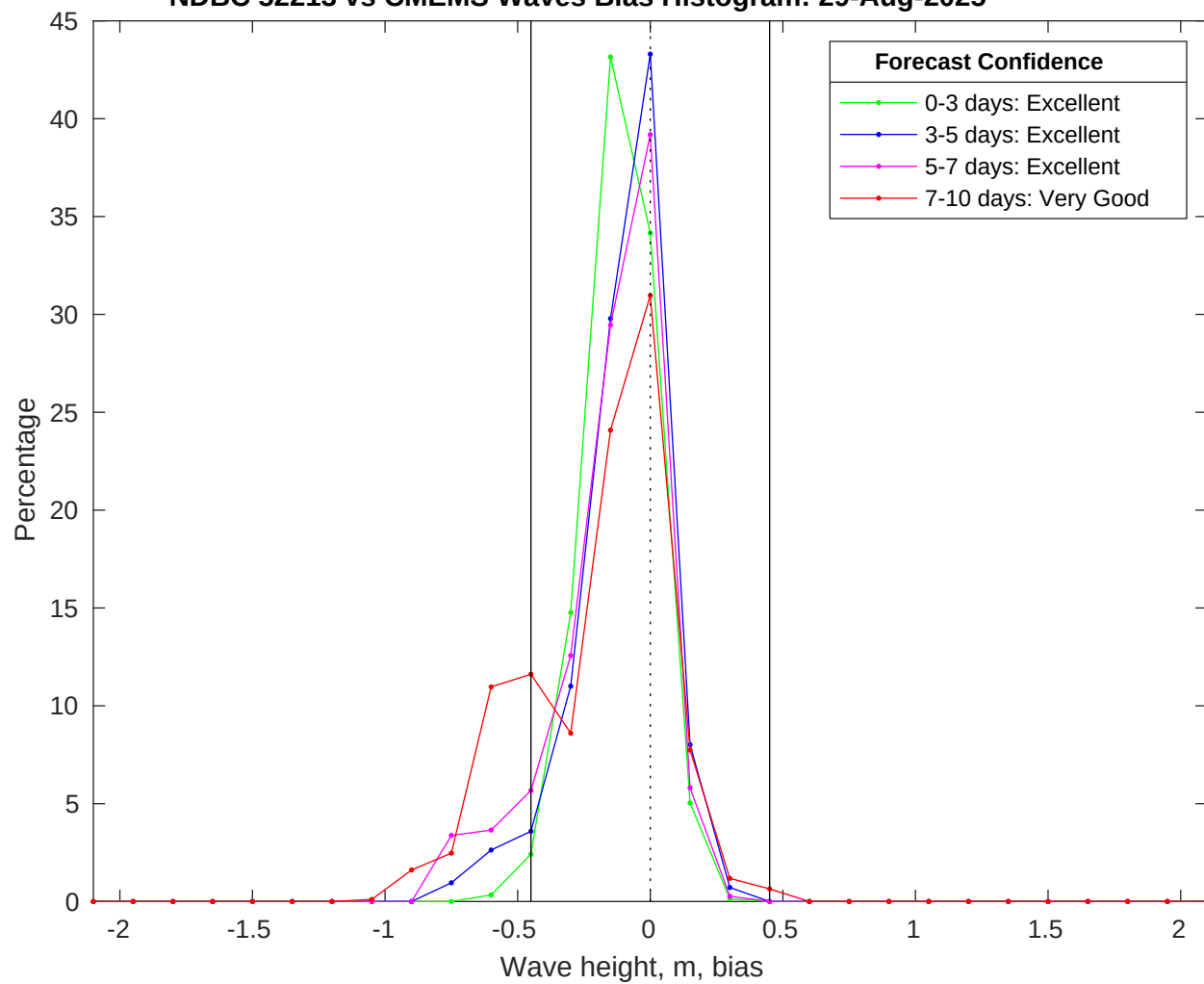
NDBC 52213 vs CMEMS Waves Bias Histogram: 29-Aug-2025
