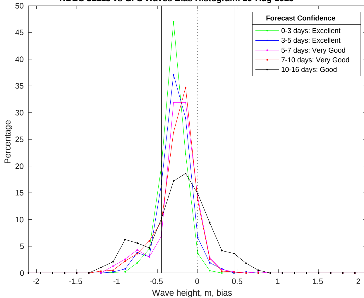
NDBC 52213 vs GFS Waves Bias Histogram: 29-Aug-2025
