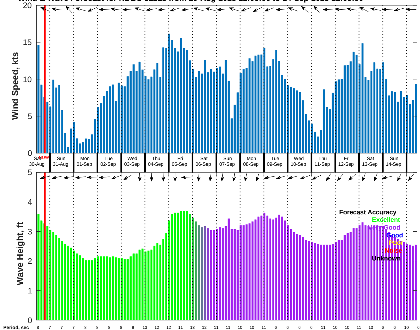
Wind & Wave Forecast for NDBC 52213 from 29-Aug-2025 11:00:00 to 14-Sep-2025 11:00:00
