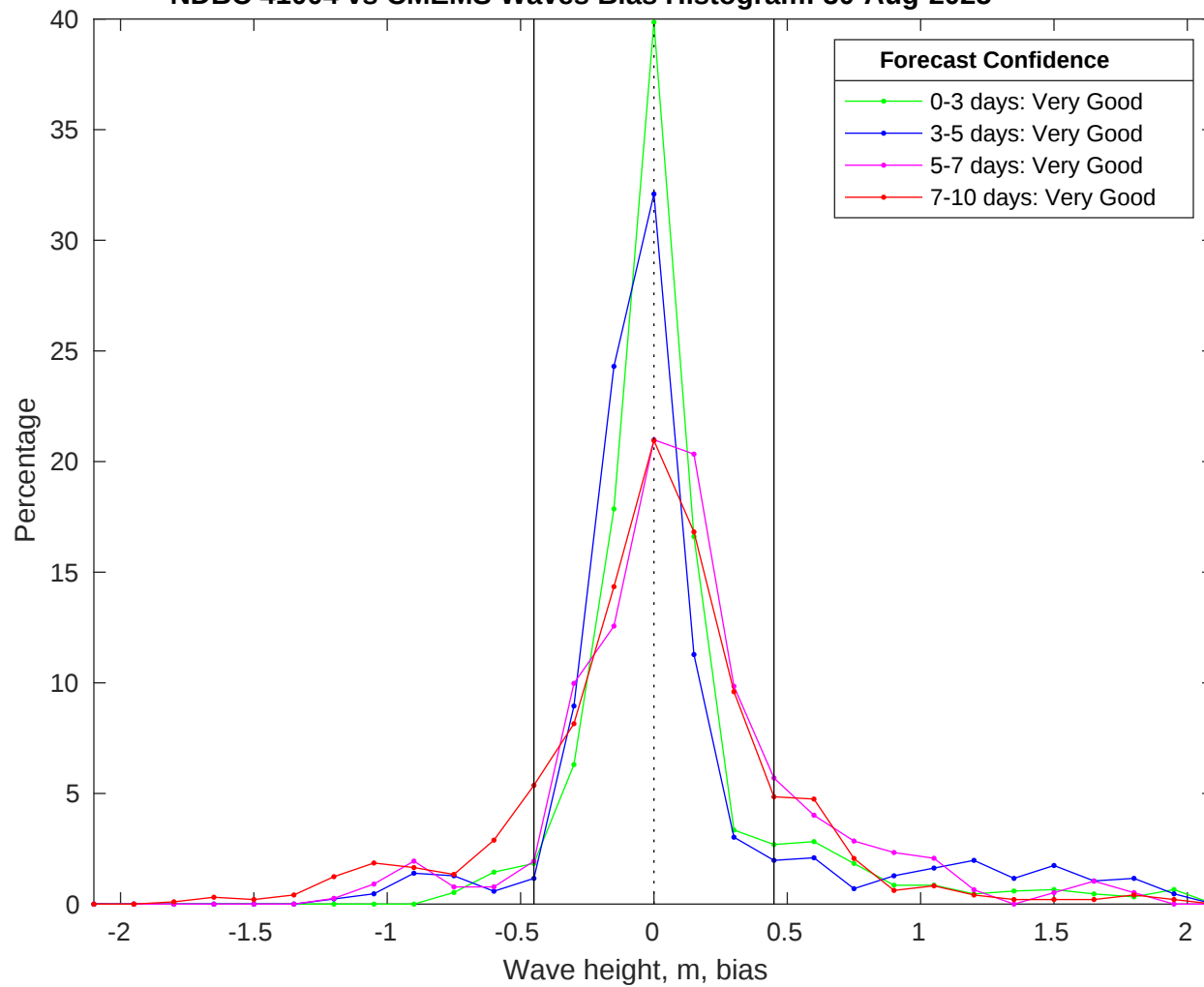
NDBC 41004 vs CMEMS Waves Bias Histogram: 30-Aug-2025
