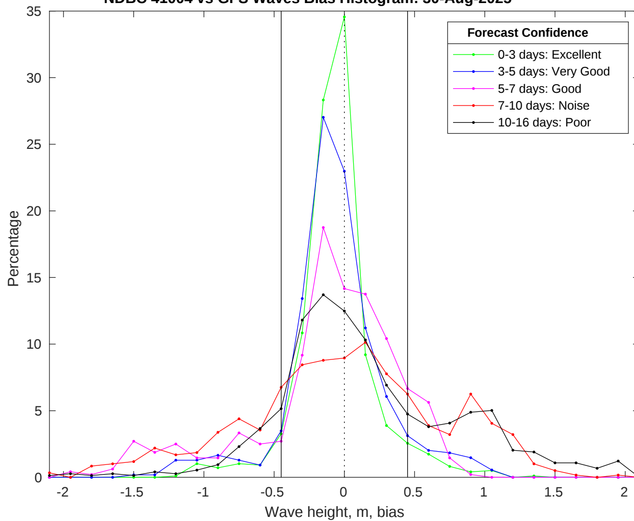
NDBC 41004 vs GFS Waves Bias Histogram: 30-Aug-2025
