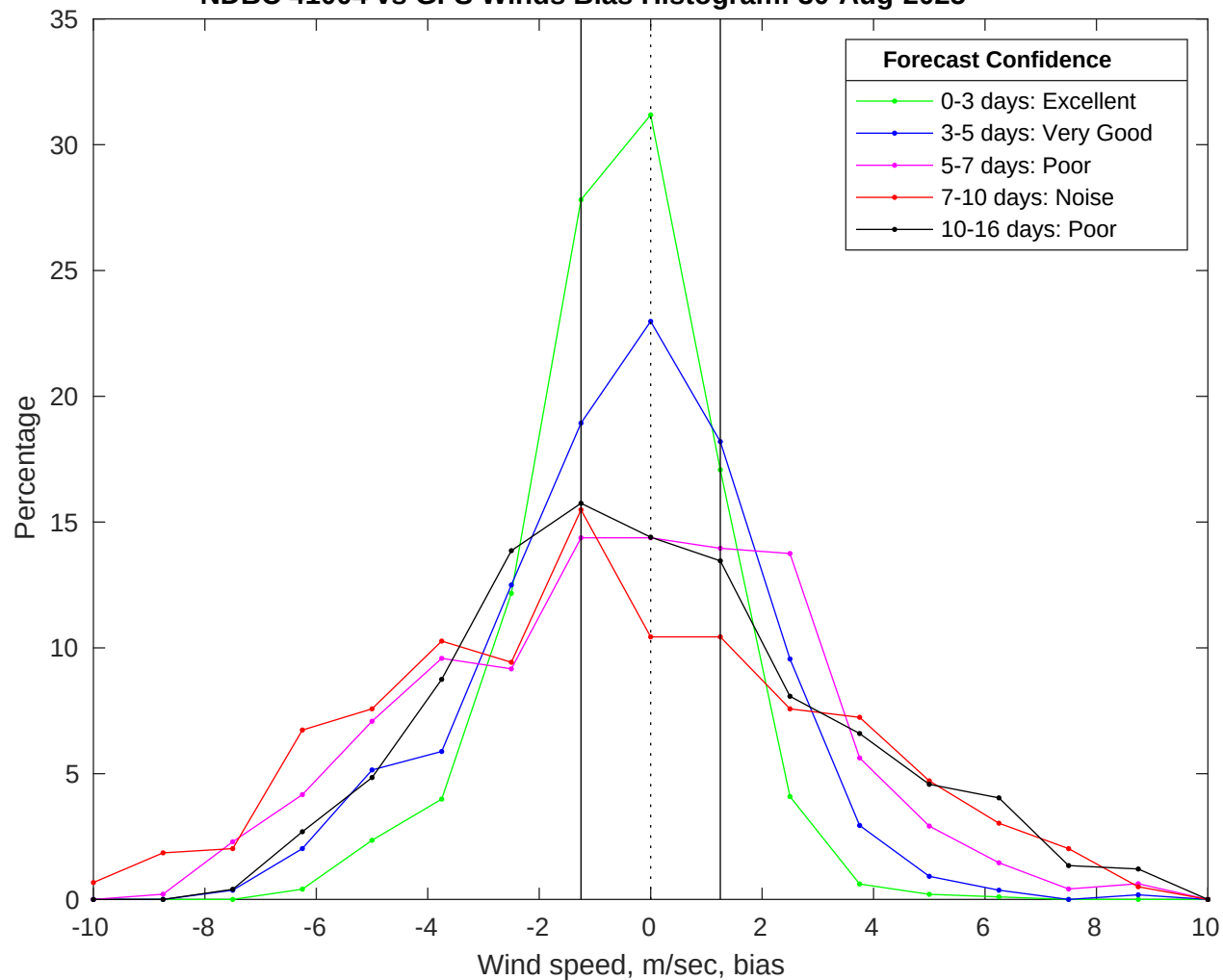
NDBC 41004 vs GFS Winds Bias Histogram: 30-Aug-2025
