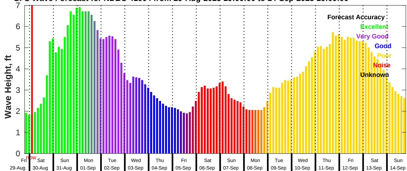
GFS Wave Forecast for NDBC 41004 from 29-Aug-2025 19:00:00 to 14-Sep-2025 19:00:00
