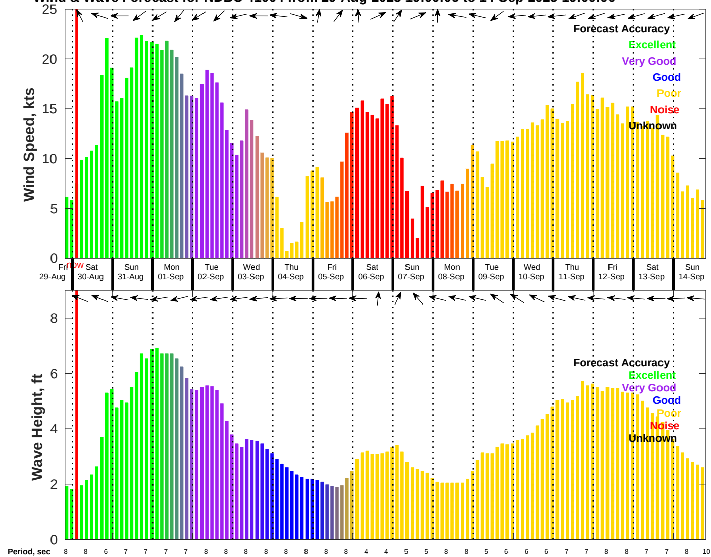
Wind & Wave Forecast for NDBC 41004 from 29-Aug-2025 19:00:00 to 14-Sep-2025 19:00:00
