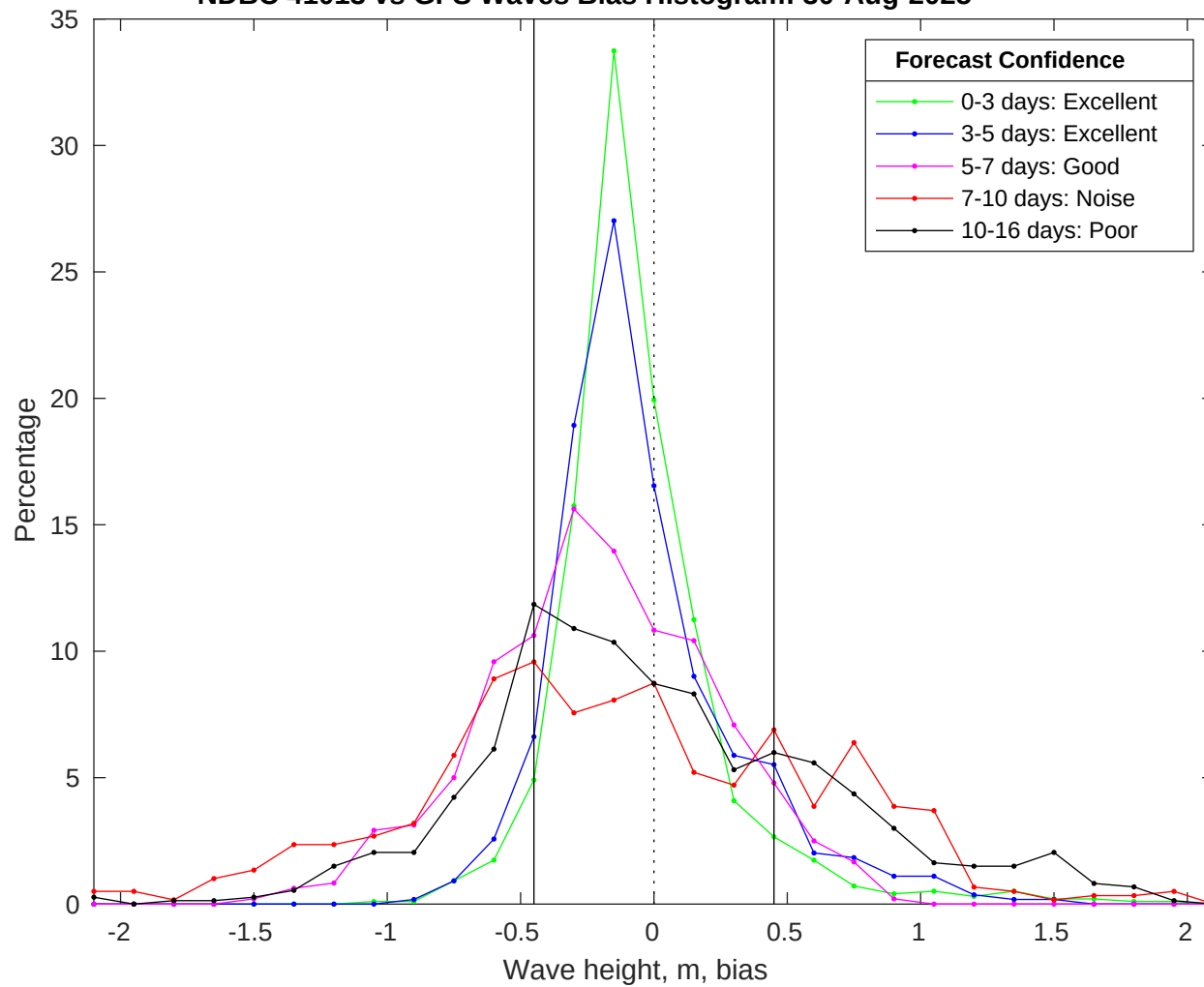
NDBC 41013 vs GFS Waves Bias Histogram: 30-Aug-2025
