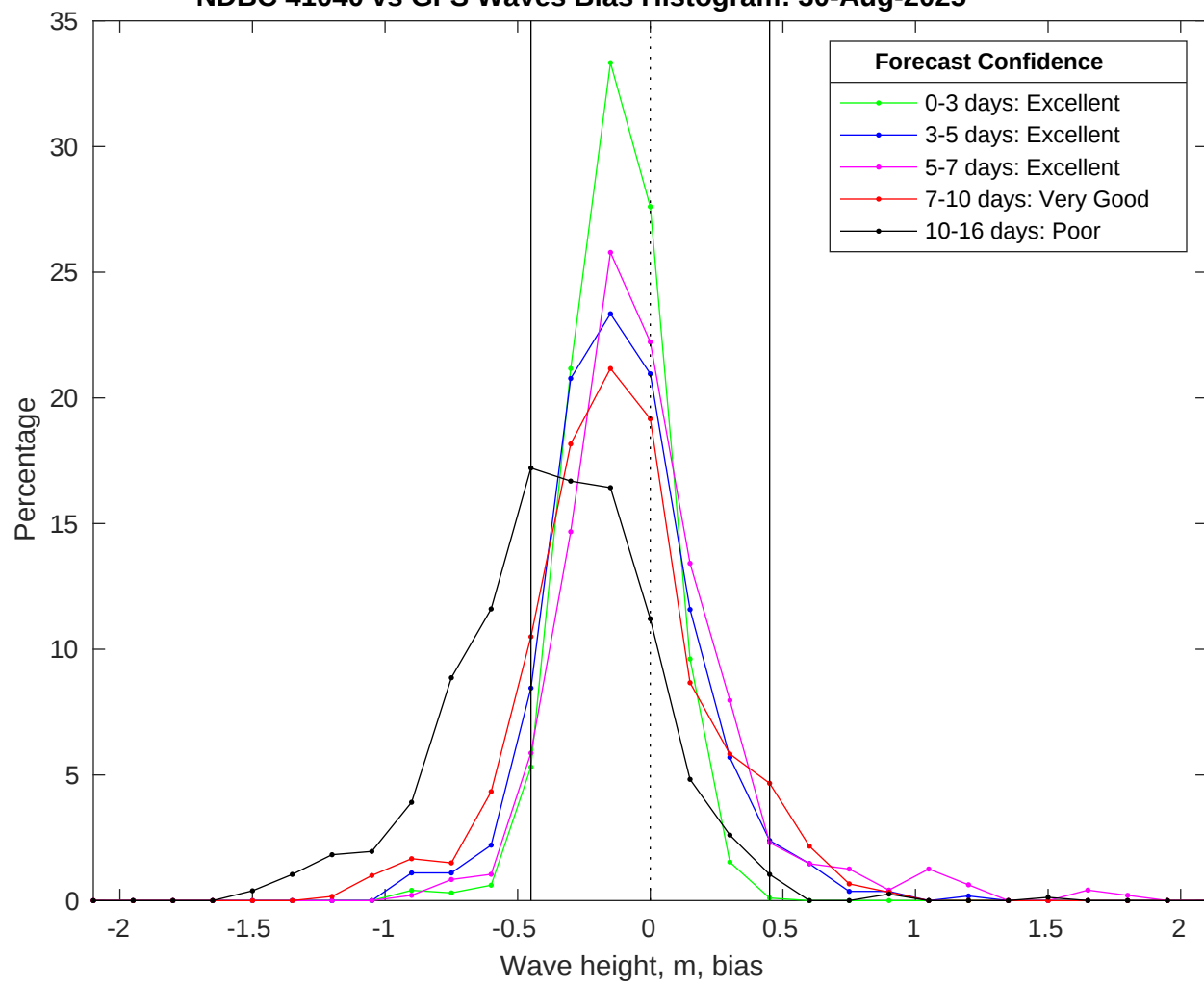
NDBC 41040 vs GFS Waves Bias Histogram: 30-Aug-2025
