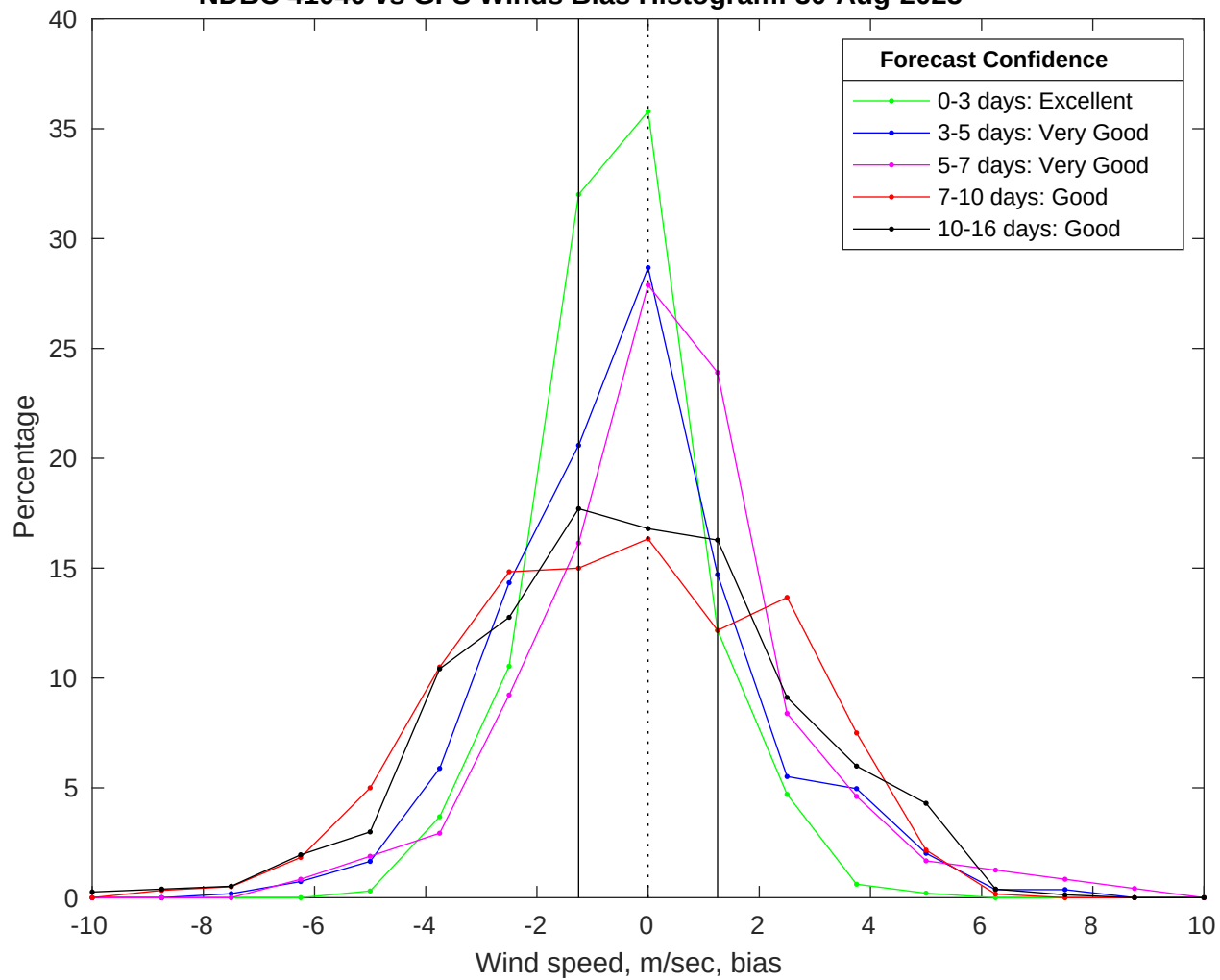
NDBC 41040 vs GFS Winds Bias Histogram: 30-Aug-2025
