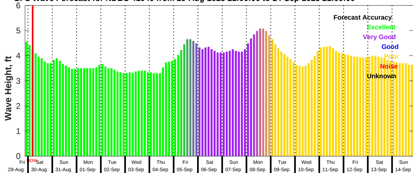
GFS Wave Forecast for NDBC 41040 from 29-Aug-2025 21:00:00 to 14-Sep-2025 21:00:00
