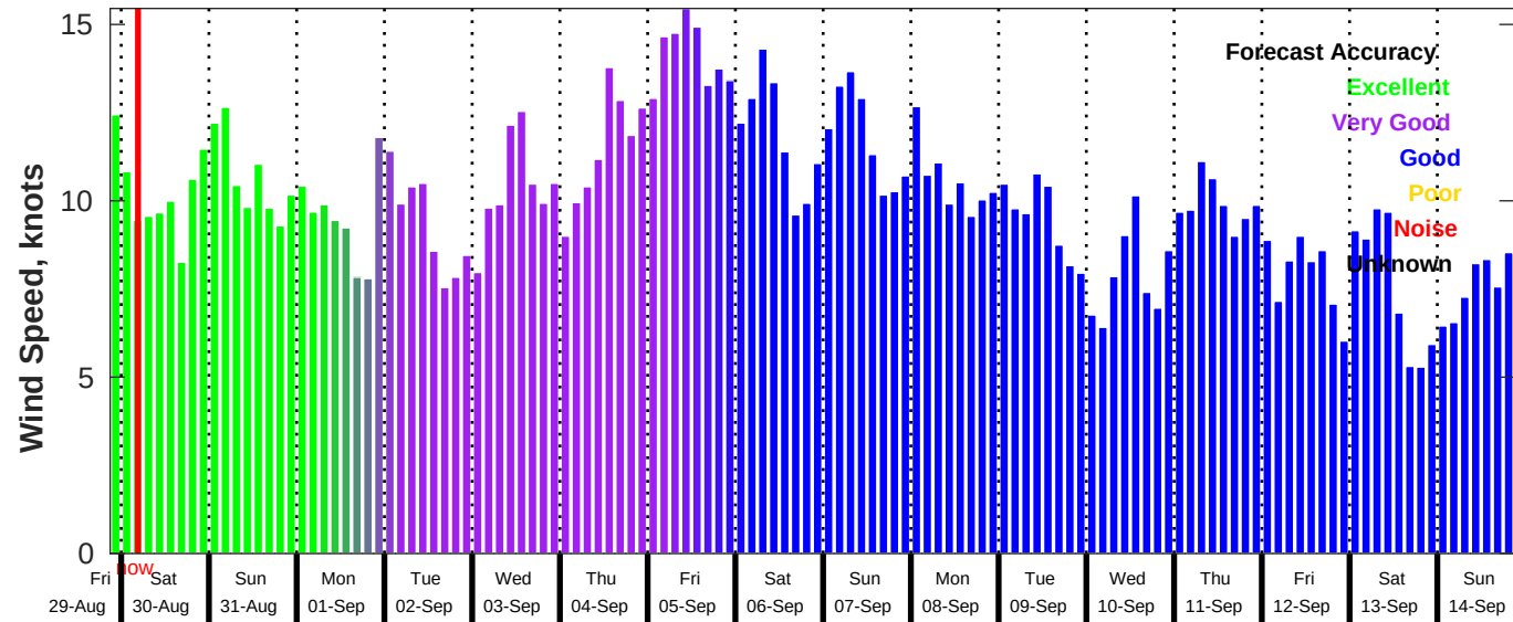
GFS Wind Speed Forecast for NDBC 41040 from 29-Aug-2025 21:00:00 to 14-Sep-2025 21:00:00
