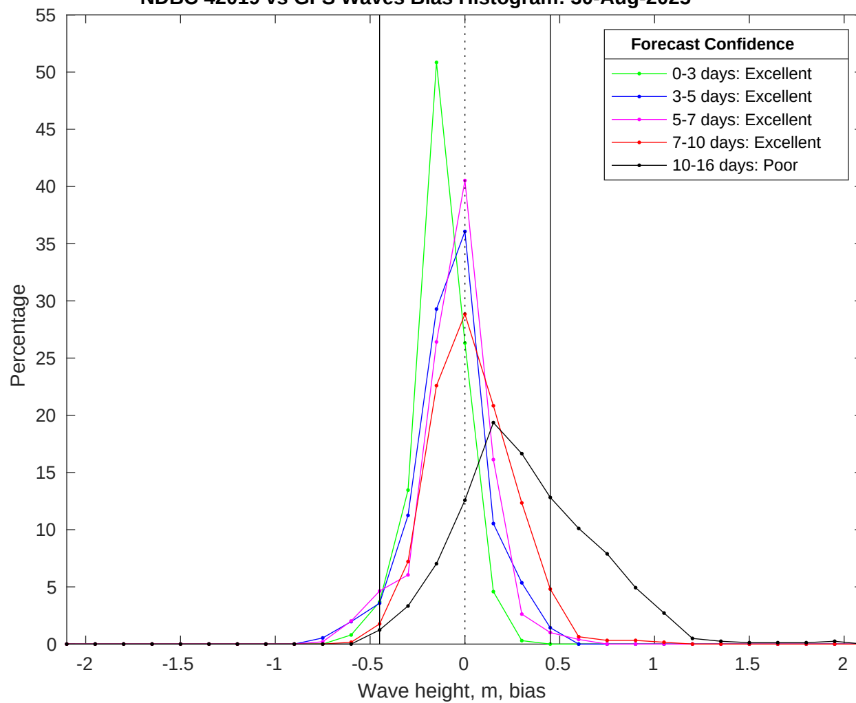
NDBC 42019 vs GFS Waves Bias Histogram: 30-Aug-2025
