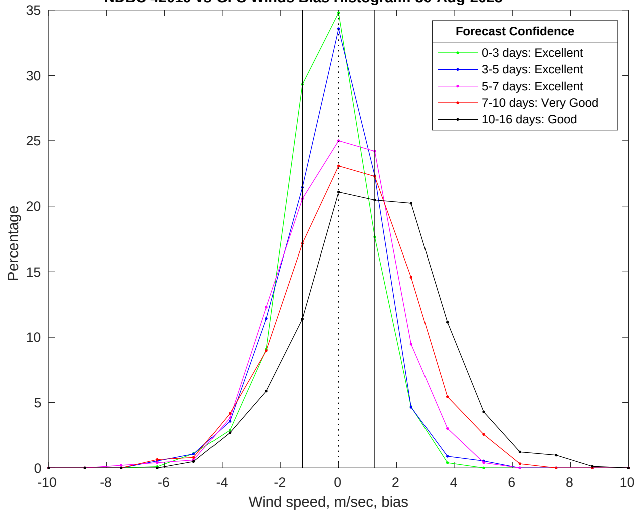
NDBC 42019 vs GFS Winds Bias Histogram: 30-Aug-2025
