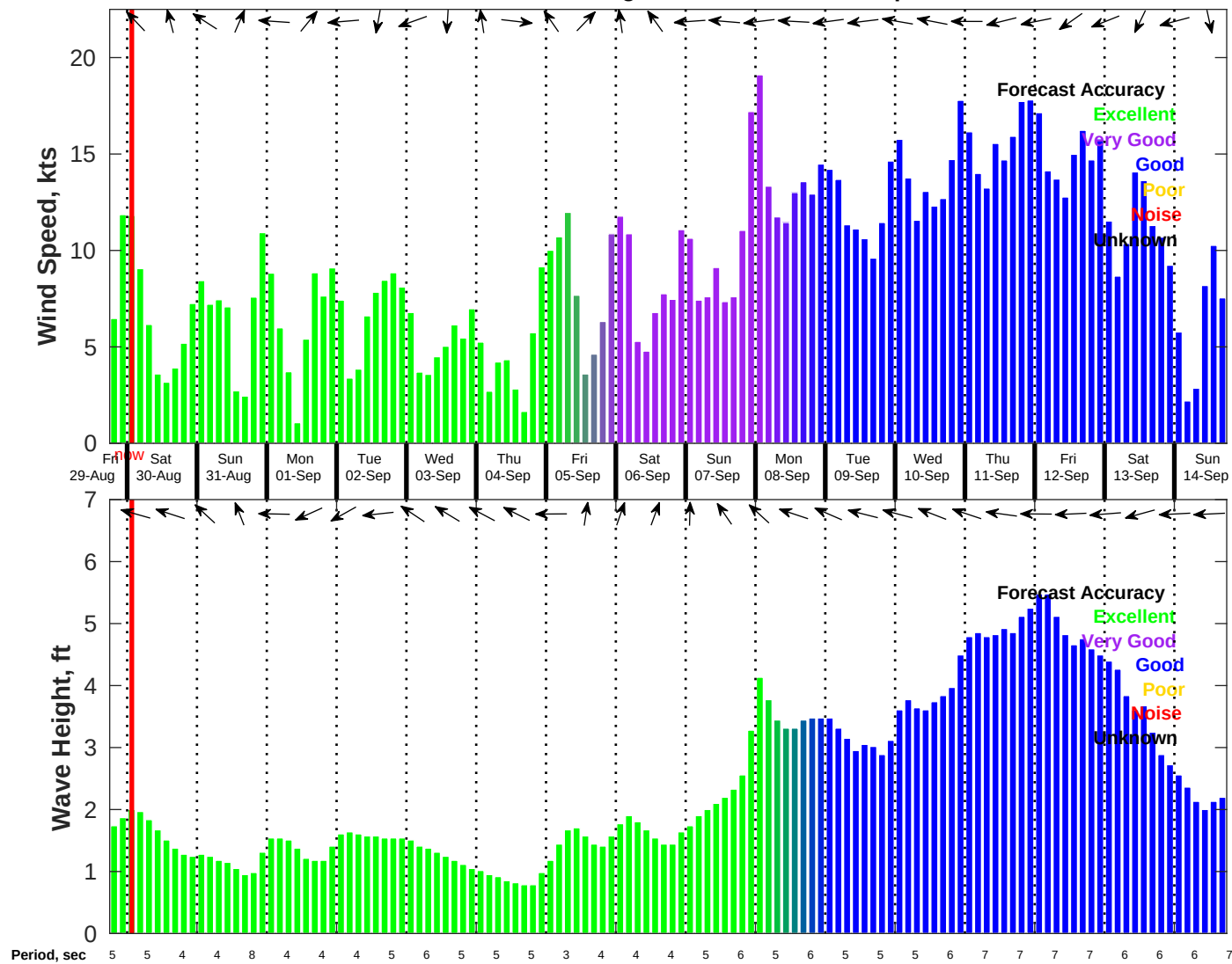
Wind & Wave Forecast for NDBC 42019 from 29-Aug-2025 18:00:00 to 14-Sep-2025 18:00:00
