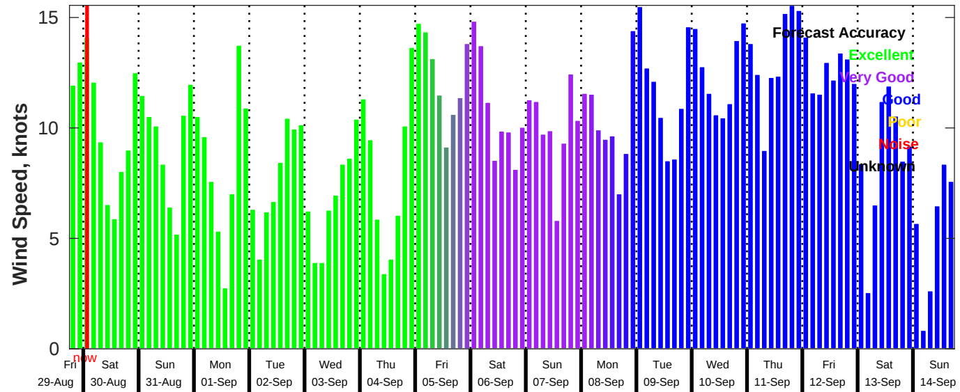
GFS Wind Speed Forecast for NDBC 42020 from 29-Aug-2025 18:00:00 to 14-Sep-2025 18:00:00
