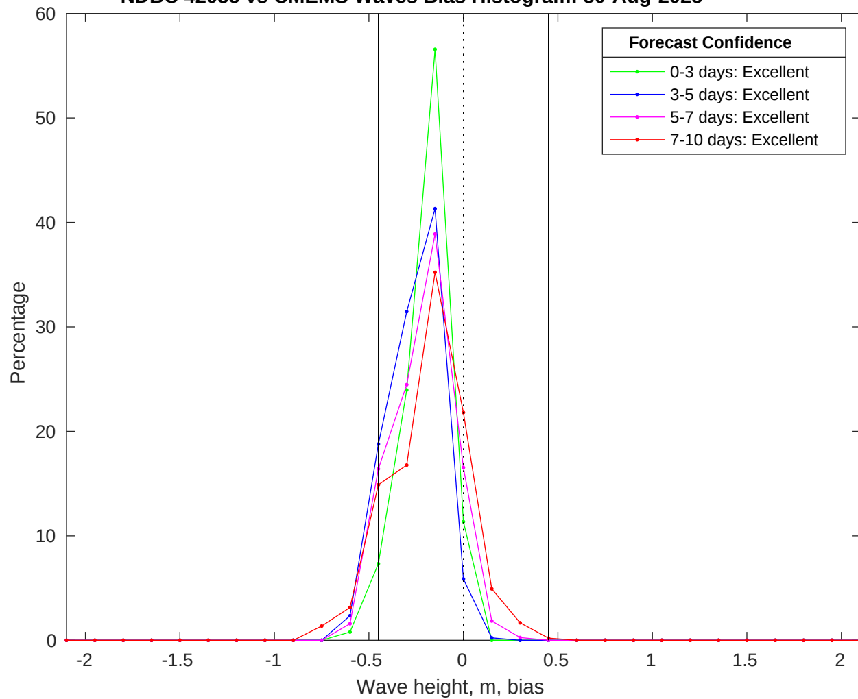
NDBC 42035 vs CMEMS Waves Bias Histogram: 30-Aug-2025
