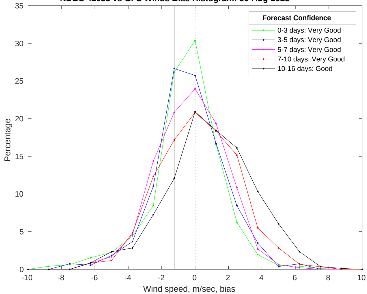
NDBC 42035 vs GFS Winds Bias Histogram: 30-Aug-2025
