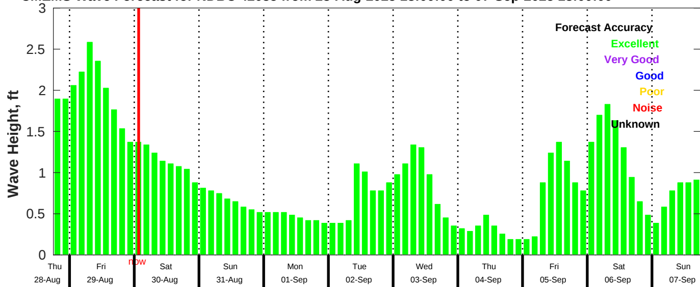
CMEMS Wave Forecast for NDBC 42035 from 28-Aug-2025 18:00:00 to 07-Sep-2025 18:00:00
