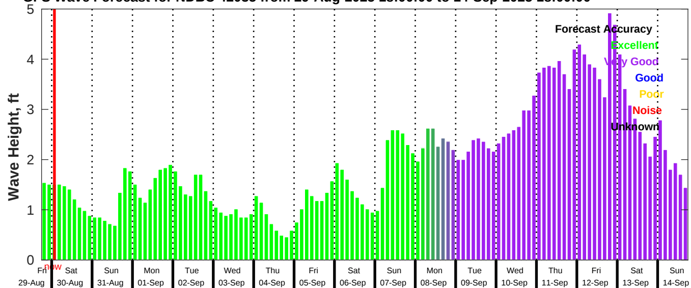
GFS Wave Forecast for NDBC 42035 from 29-Aug-2025 18:00:00 to 14-Sep-2025 18:00:00
