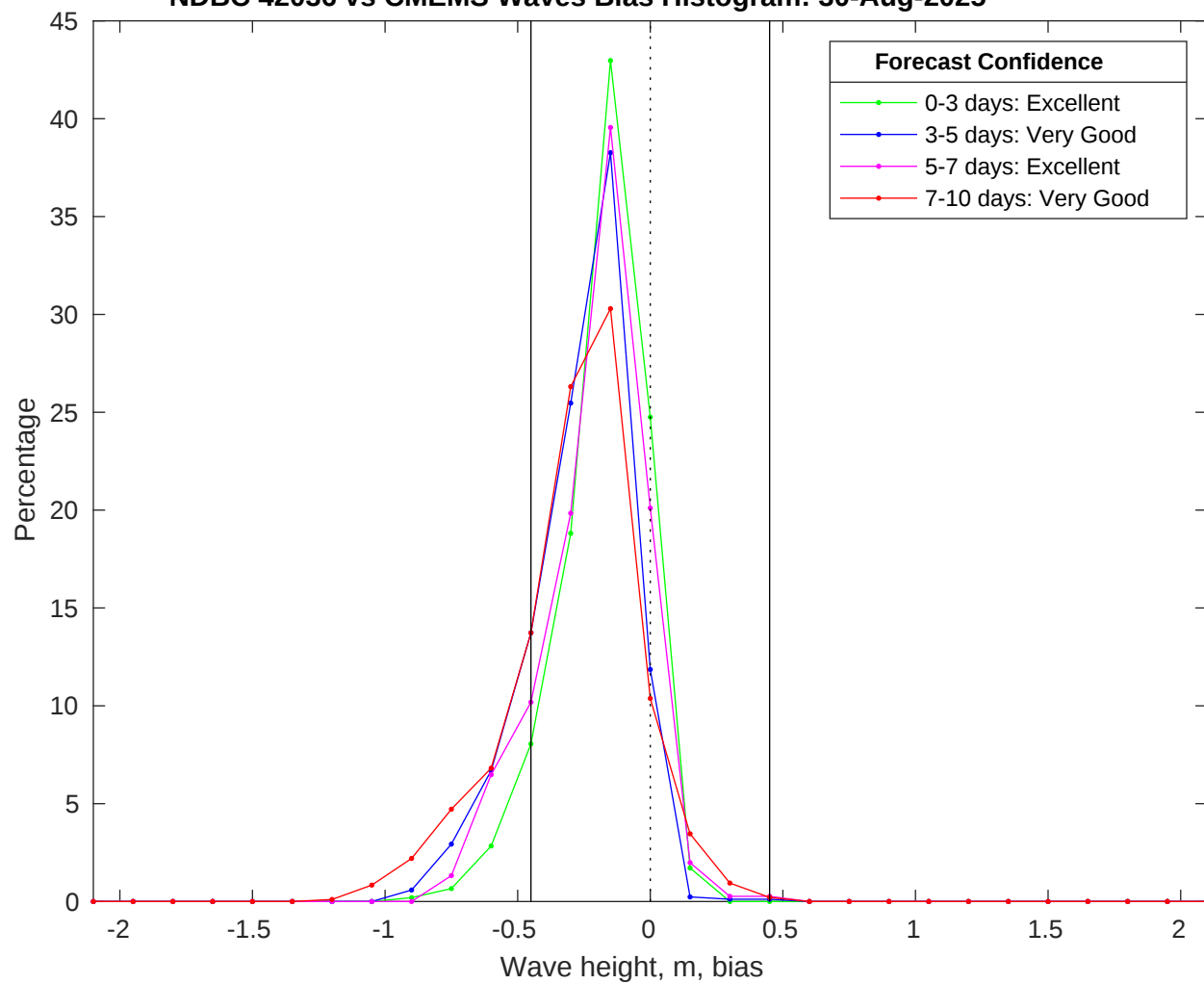
NDBC 42036 vs CMEMS Waves Bias Histogram: 30-Aug-2025
