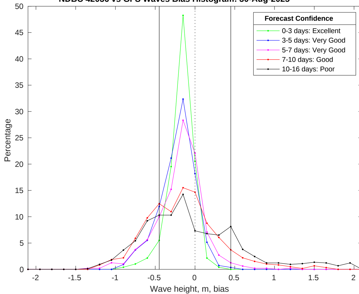
NDBC 42036 vs GFS Waves Bias Histogram: 30-Aug-2025
