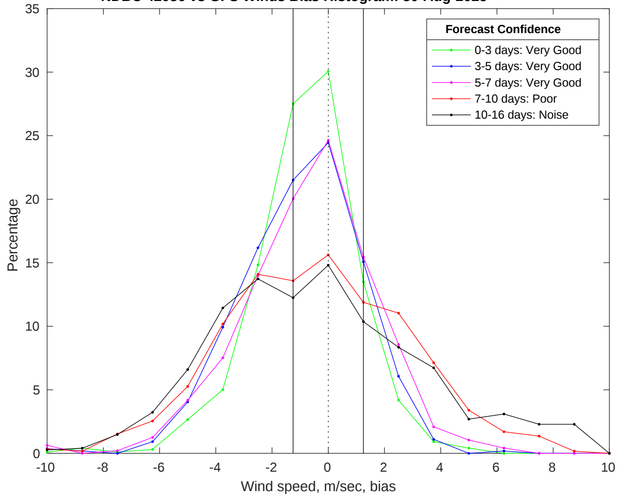
NDBC 42036 vs GFS Winds Bias Histogram: 30-Aug-2025
