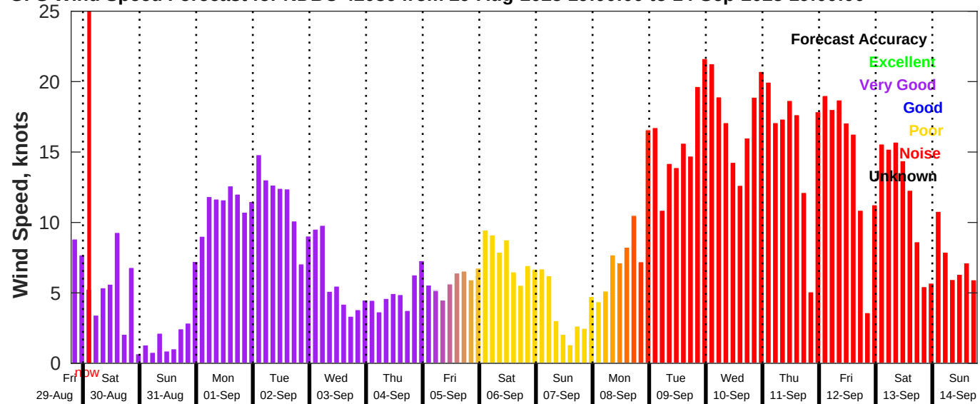
GFS Wind Speed Forecast for NDBC 42036 from 29-Aug-2025 19:00:00 to 14-Sep-2025 19:00:00
