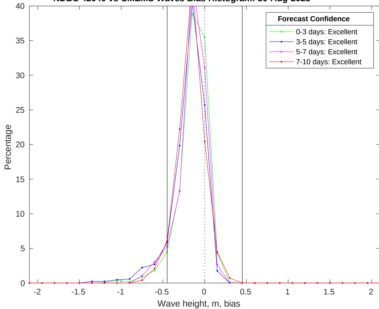
NDBC 42040 vs CMEMS Waves Bias Histogram: 30-Aug-2025
