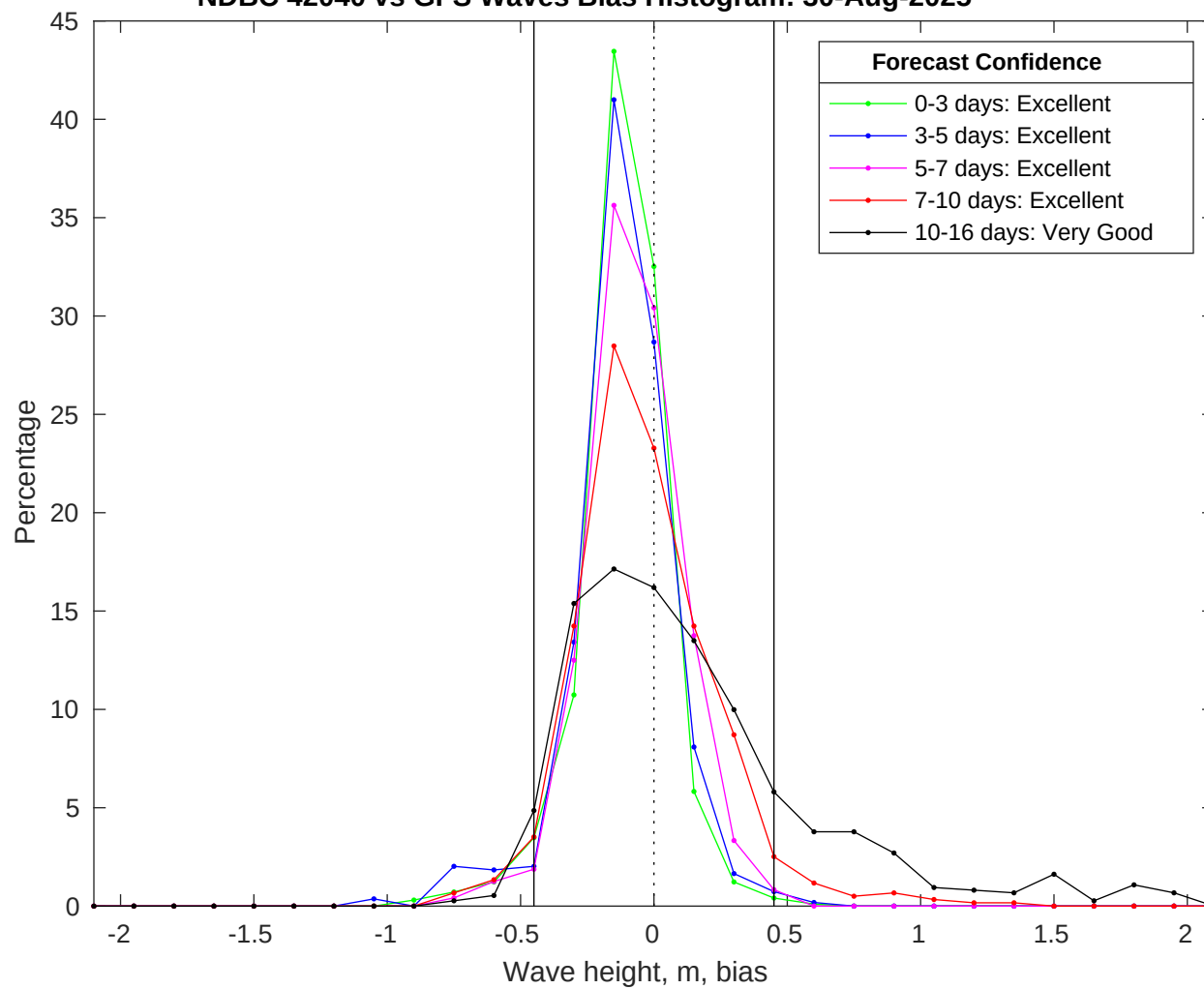
NDBC 42040 vs GFS Waves Bias Histogram: 30-Aug-2025
