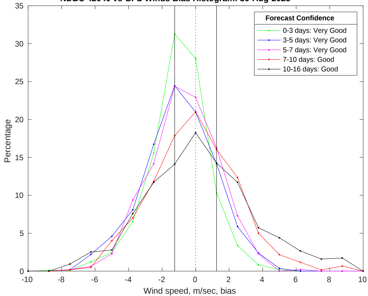
NDBC 42040 vs GFS Winds Bias Histogram: 30-Aug-2025
